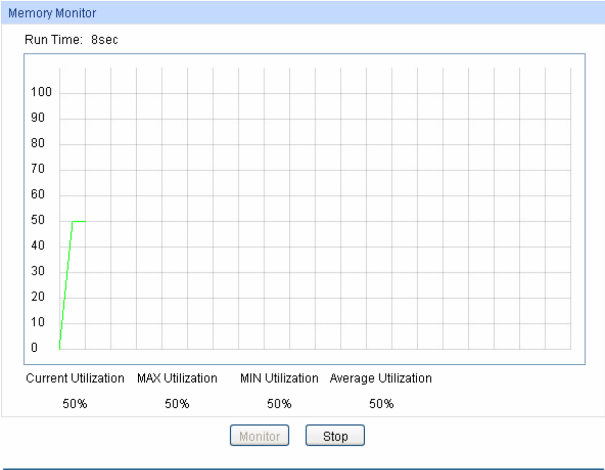
Figure 11-2 Memory Monitor
